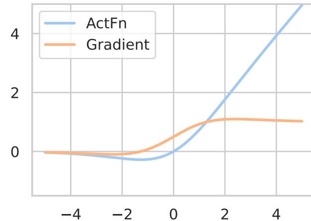
Swish
