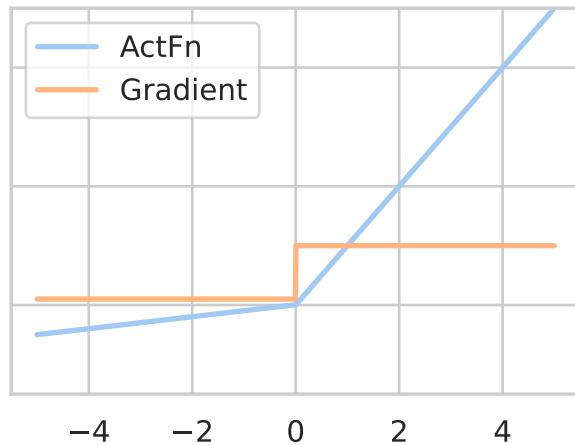
LeakyReLU
