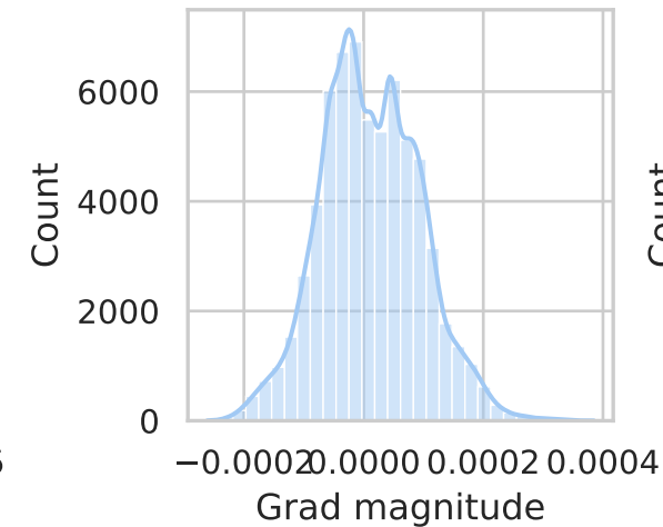
layers.4.weight
