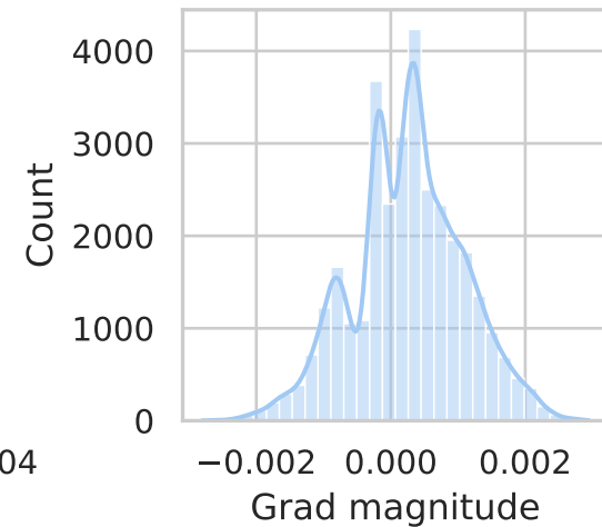
layers.6.weight
