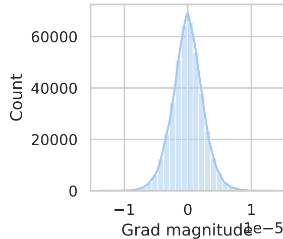
layers.0.weight
