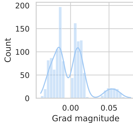
layers.8.weight
