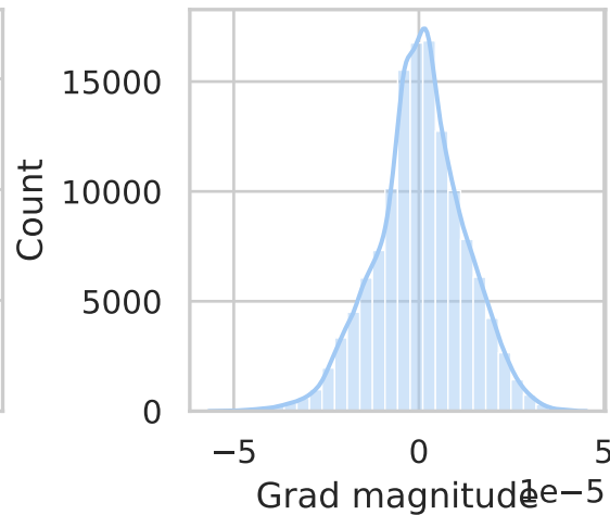
layers.2.weight
