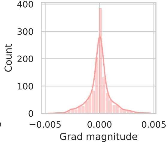
layers.8.weight
