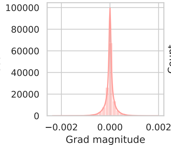
layers.2.weight
