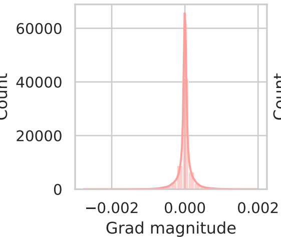
layers.4.weight
