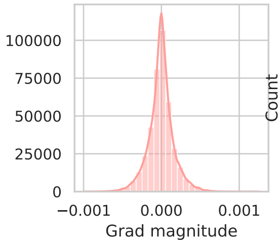
layers.0.weight
