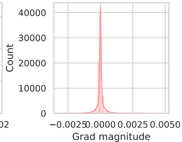
layers.6.weight
